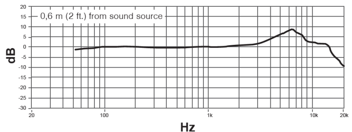
Frequency Response
